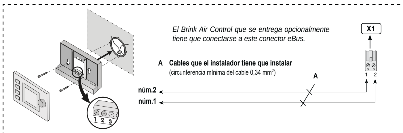
conector Ebus bipolar
