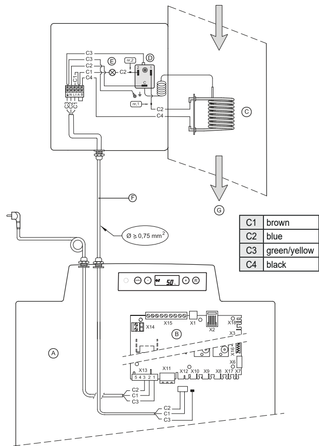
Preheater
