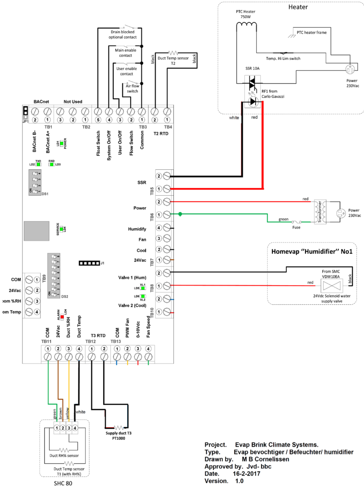
Wiring diagram Evap
